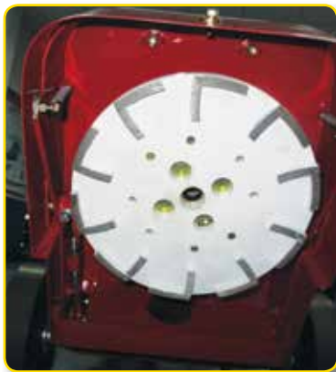
10" Grinding Plate and Segment - Ideal for Grinding of Wet or Dry Concrete Surfaces
